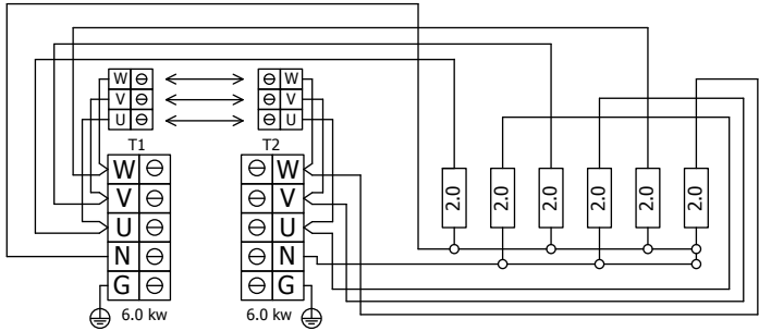
DRFT6-120NS-CNR 12,0 kW
