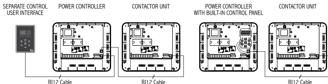
Fig. 4 Installation of separate control panel with power controller and contactor unit
